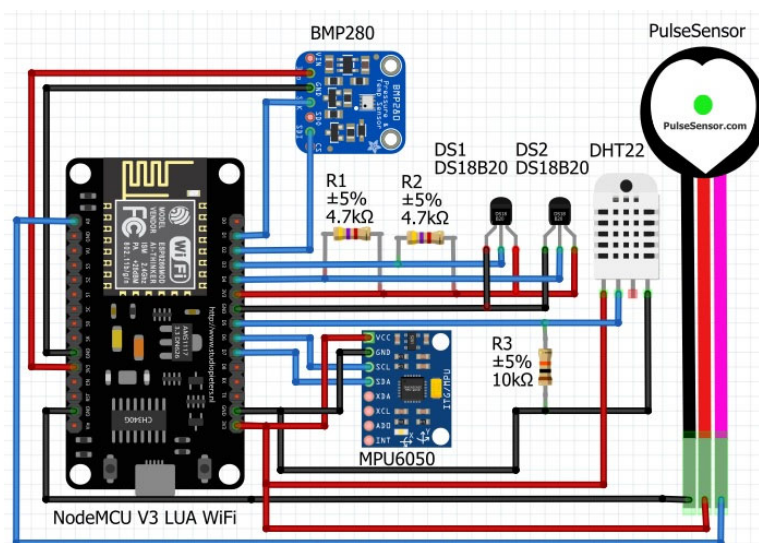
Figure 7.18. Smart vest controllers assembly scheme
