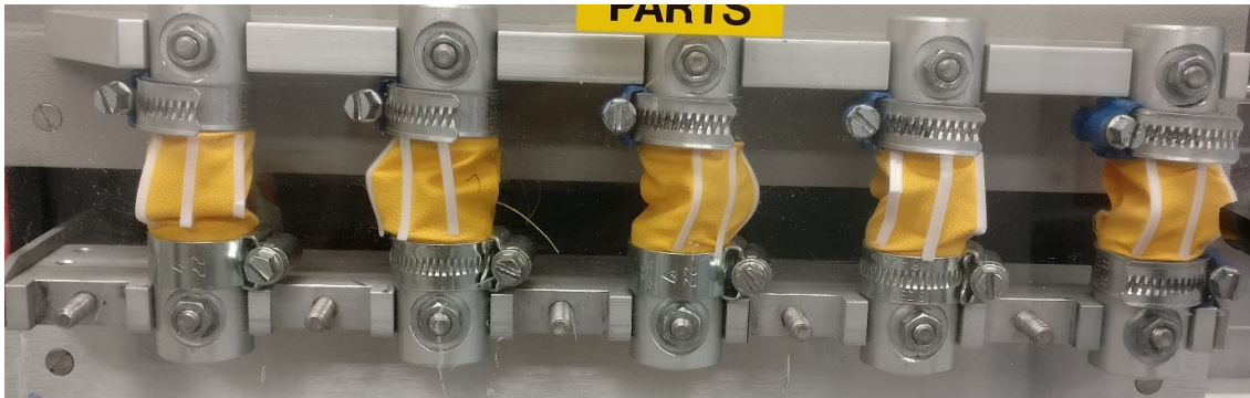
Figure 6.2. Flexing test of standard PLA
