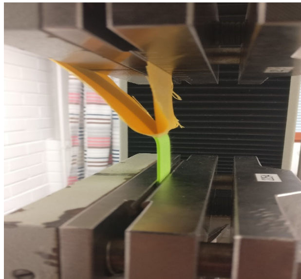
Figure 6.1. Printed TPU peeling test sample
