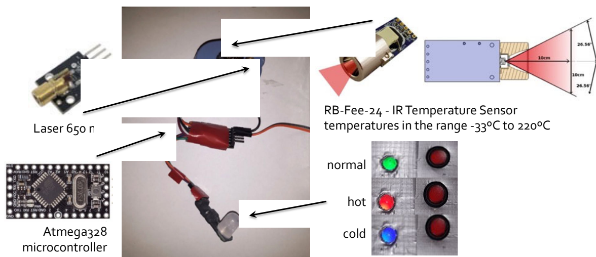
Figure 7.26. The unit for remote surface temperature control
