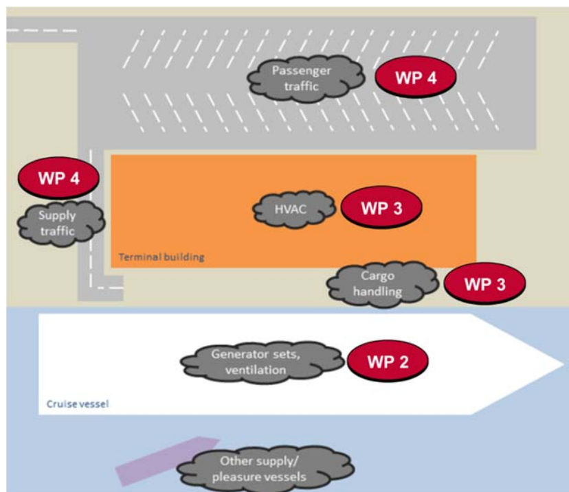
Figure 14: Emission sources of a typical cruise terminal and connection to project WPs 16
