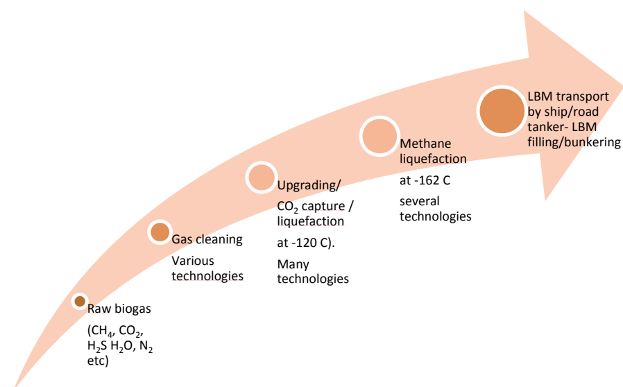
Figure 4. The major steps from biogas towards LBM. For further explanation, see text.
